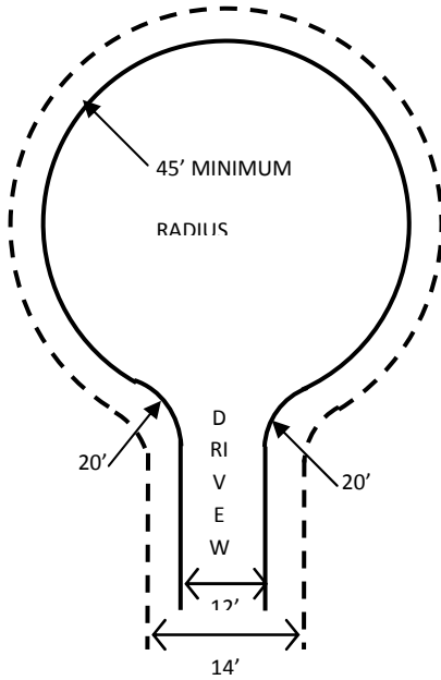
CLEARANCE CUL-DE-SAC
